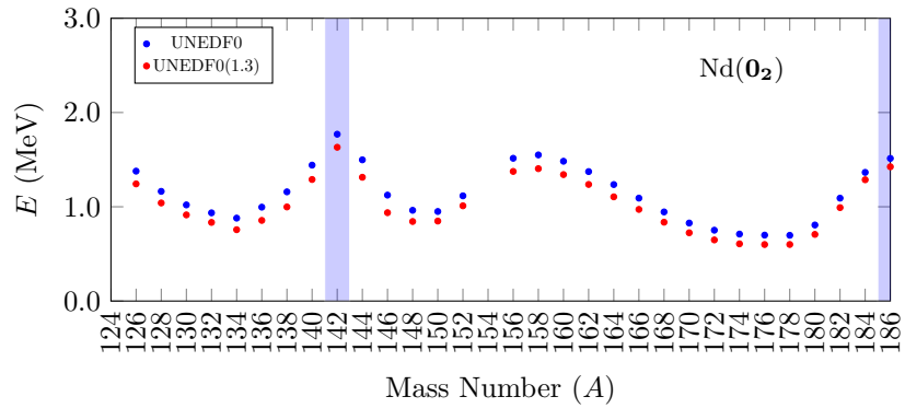
Figure 8: Bohr Hamiltonian calculations for the 0_2 states of the Nd isotopic chain with the UNEDF0 functional.
