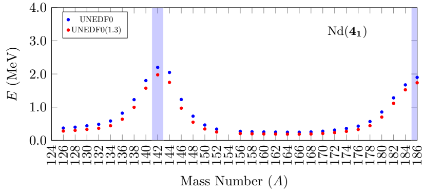
Figure 3: Bohr Hamiltonian calculations for the 4_1 states of the Nd isotopic chain with the UNEDF0 functional.
