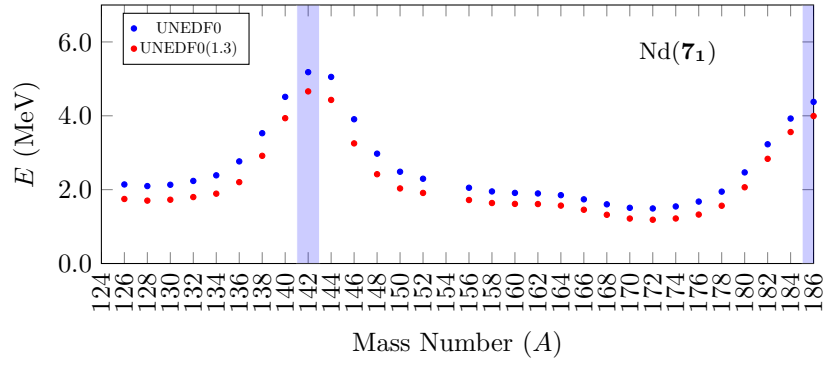
Figure 6: Bohr Hamiltonian calculations for the 7_1 states of the Nd isotopic chain with the UNEDF0 functional.
