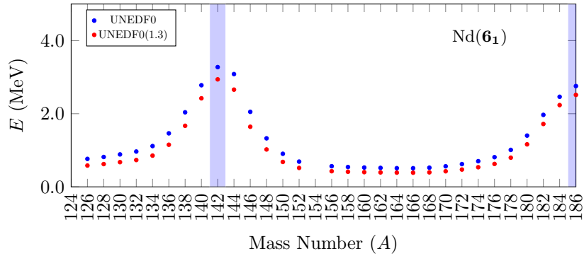
Figure 5: Bohr Hamiltonian calculations for the 6_1 states of the Nd isotopic chain with the UNEDF0 functional.
