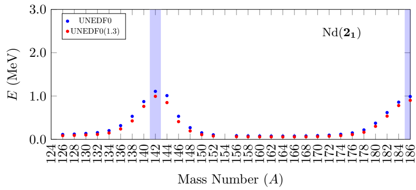
Figure 1: Bohr Hamiltonian calculations for the 2_1 states of the Nd isotopic chain with the UNEDF0 functional.
