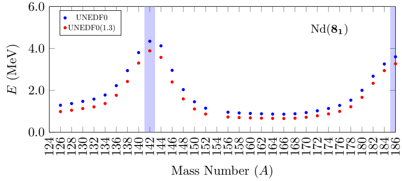
Figure 7: Bohr Hamiltonian calculations for the 8_1 states of the Nd isotopic chain with the UNEDF0 functional.
