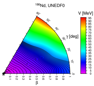
Figure 9: Nd isotopic chain potential energy surfaces.
