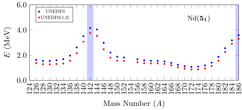
Figure 4: Bohr Hamiltonian calculations for the 5_1 states of the Nd isotopic chain with the UNEDF0 functional.
