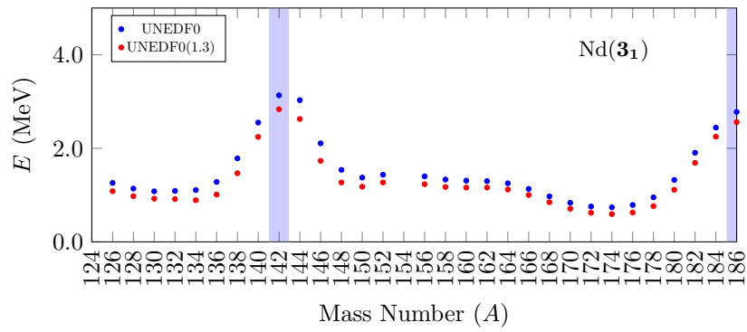
Figure 2: Bohr Hamiltonian calculations for the 3_1 states of the Nd isotopic chain with the UNEDF0 functional.
